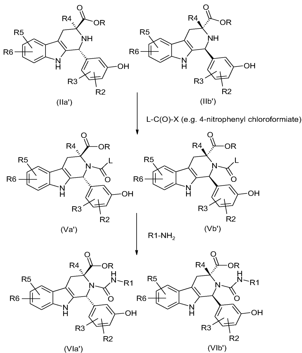
Reaction scheme 4:
